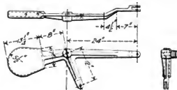
Figs. 674-676. Ashpan Bell Crank with Counterweight.
